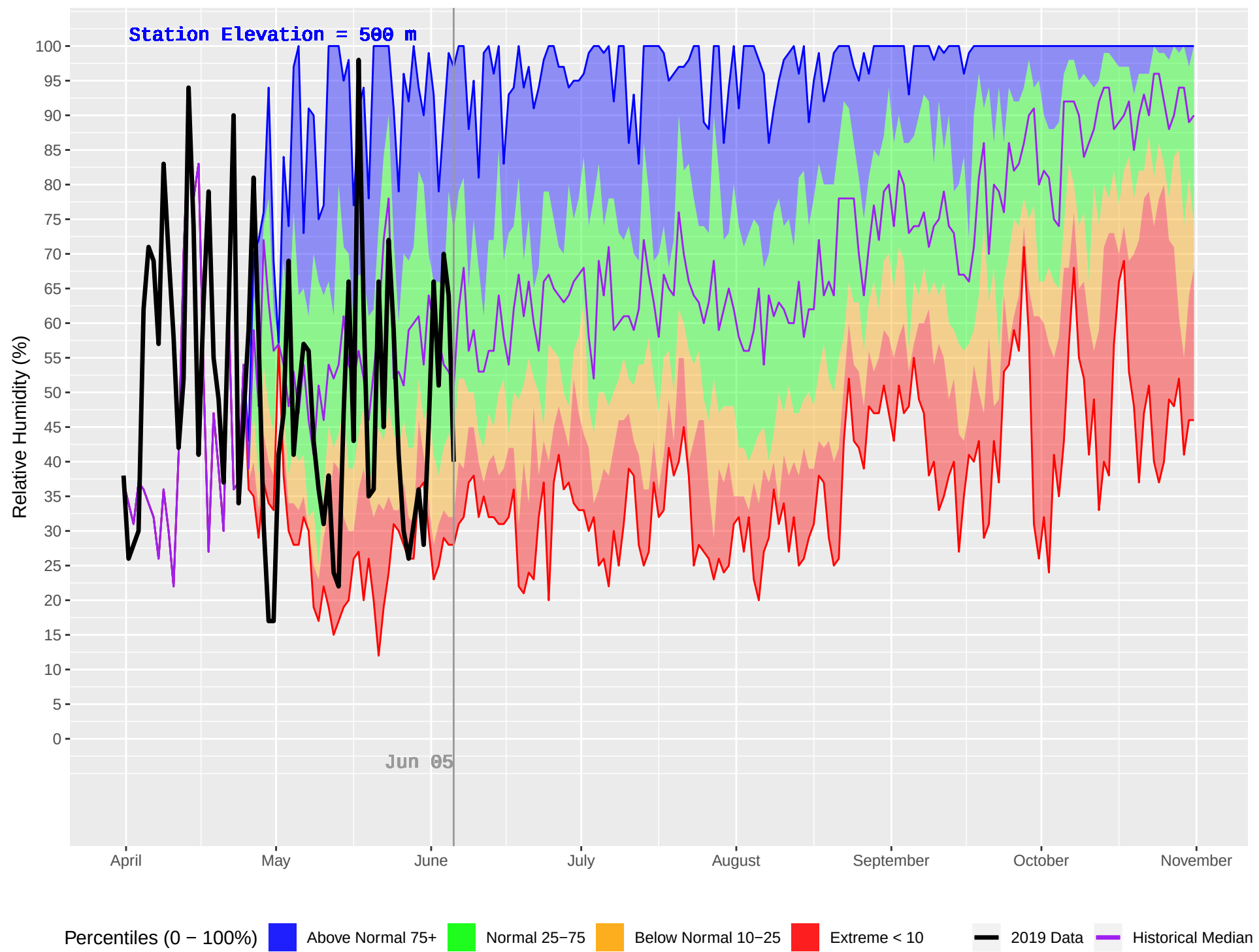
CRANBERRY (433) : Historical (1995–2018) and Current (2019) Daily Relative Humidity
