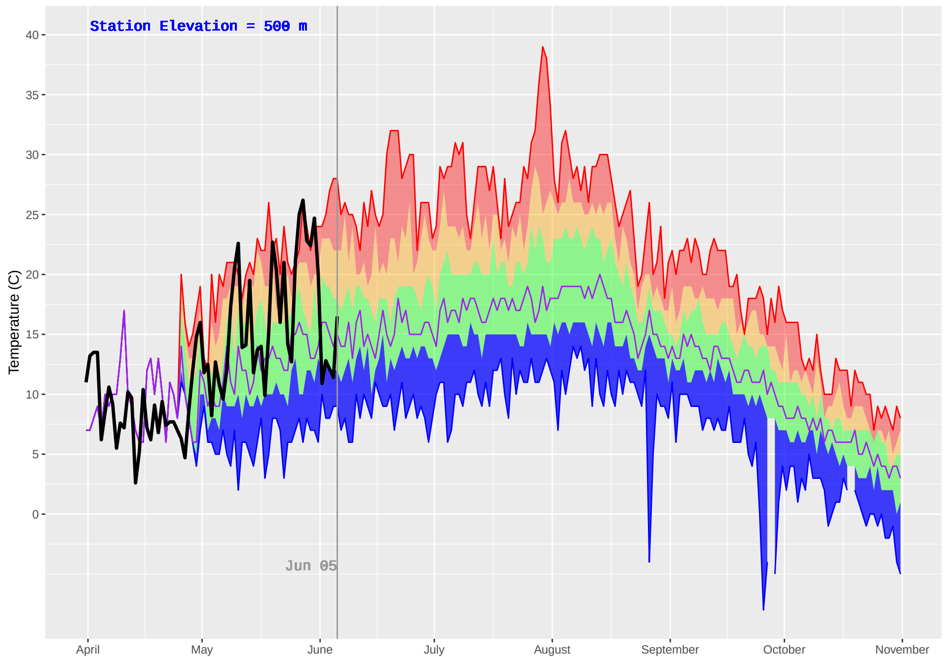
CRANBERRY (433) : Historical (1995–2018) and Current (2019) Daily Temperature
