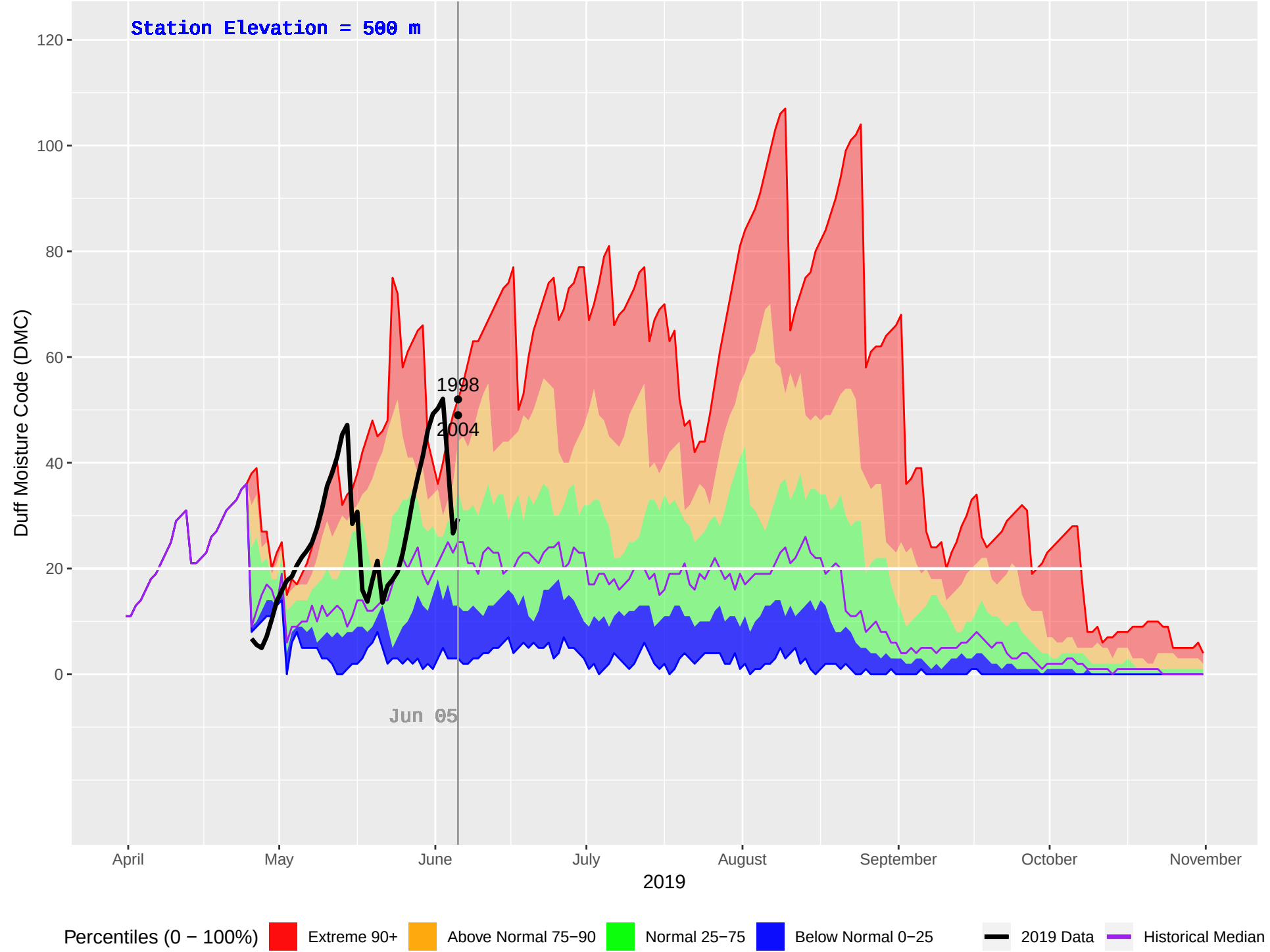
CRANBERRY (433) : Historical (1995–2018), Current (2019) Daily Duff Moisture Code (DMC)
