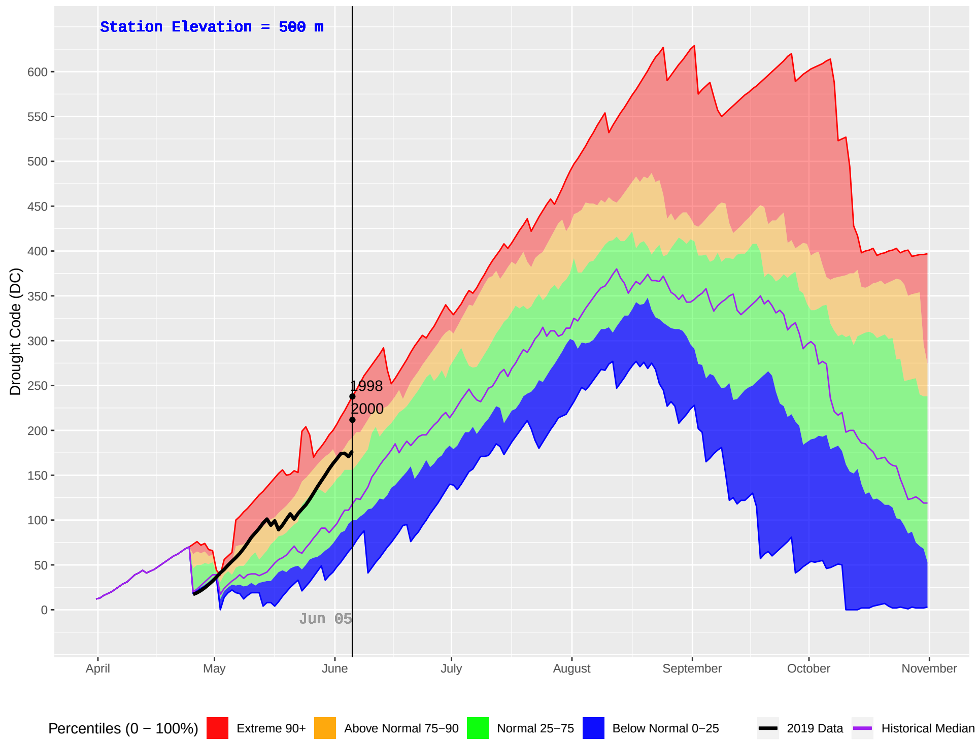
CRANBERRY (433) : Historical (1995–2018) and Current (2019) Daily Drought Code (DC)
