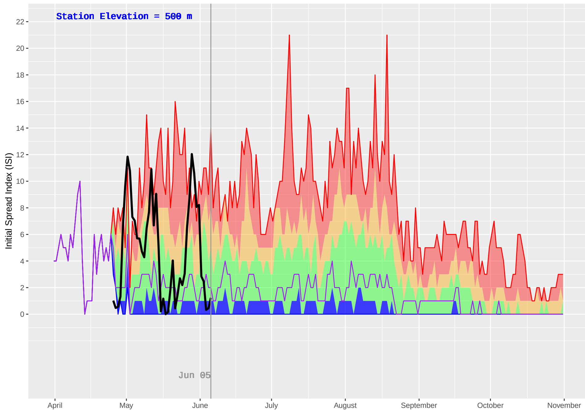
CRANBERRY (433) : Historical (1995–2018) and Current (2019) Daily Initial Spread Index (ISI)
