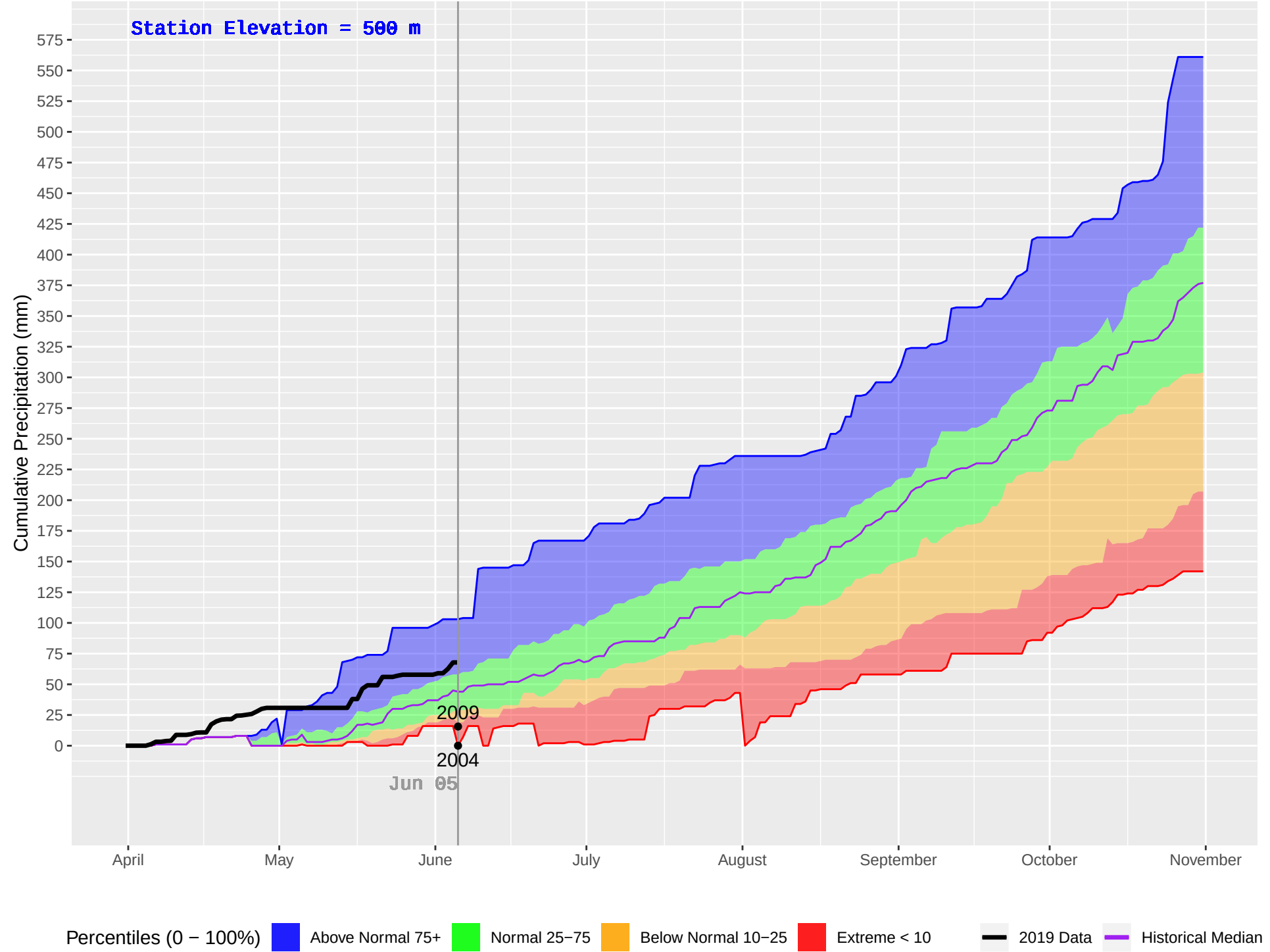
CRANBERRY (433) : Historical (1995–2018), Current (2019) Daily Cumulative Precipitation
