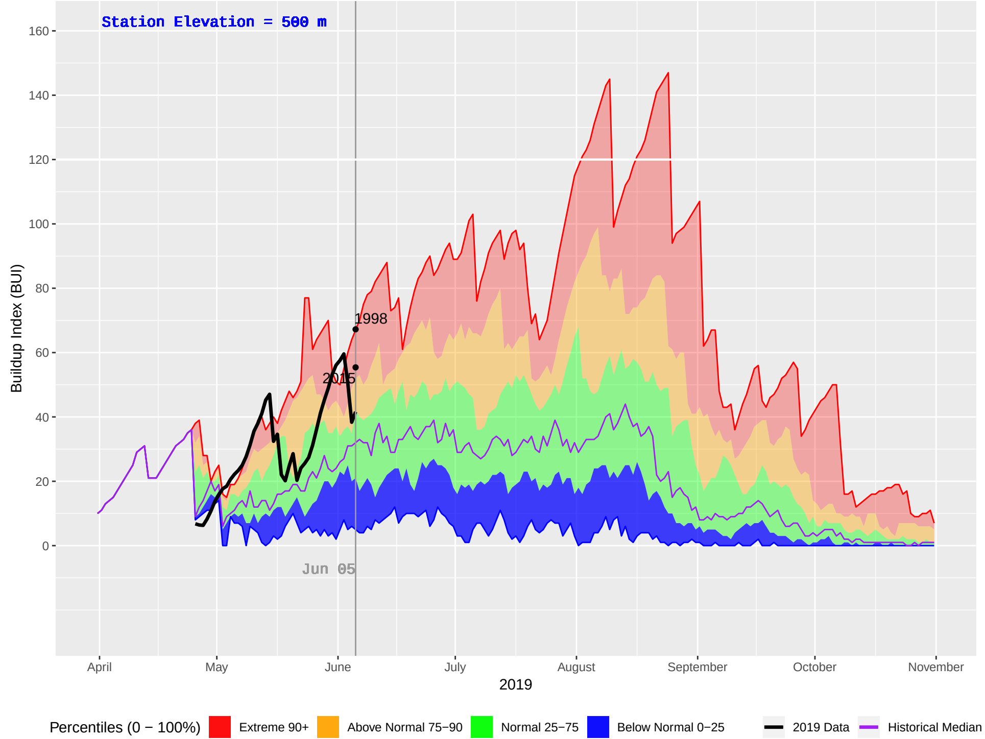
CRANBERRY (433) : Historical (1995–2018), Current (2019) Daily Buildup Index (BUI)
