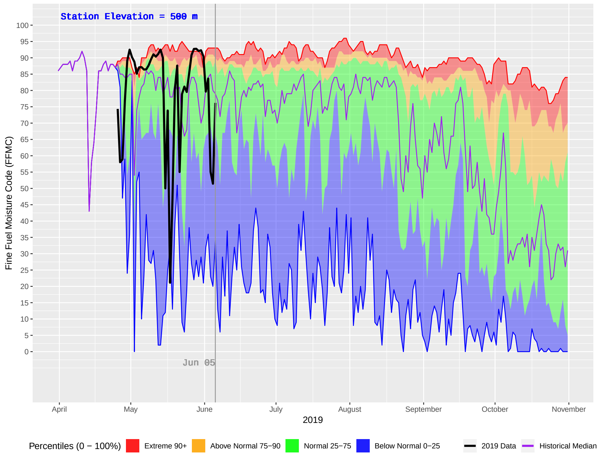
CRANBERRY (433) : Historical (1995–2018) and Current (2019) Daily Fine Fuel Moisture Code (FFMC)
